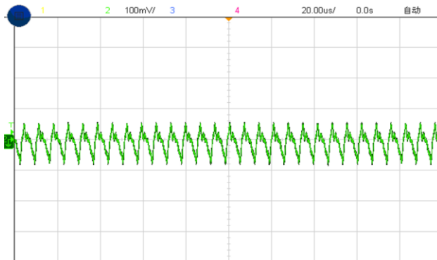
Figure 7, Output ripple & noise ( I_{out} = 3\text{A} )
