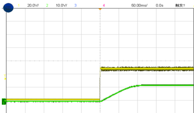
Figure 6, Output voltage established ( I_{out} = 3\text{A} )
