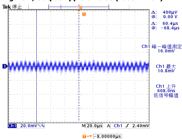
Figure 7, Output ripple & noise (Iout = 1.5A)
