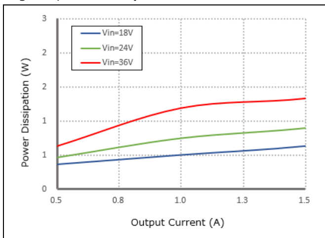
Figure 2, Power dissipation
