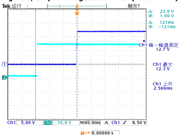
Figure 6, Output voltage established (Iout = 1.5A)
