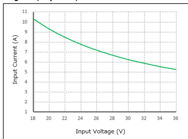
Figure 3, Input V-I, Iout=15A
