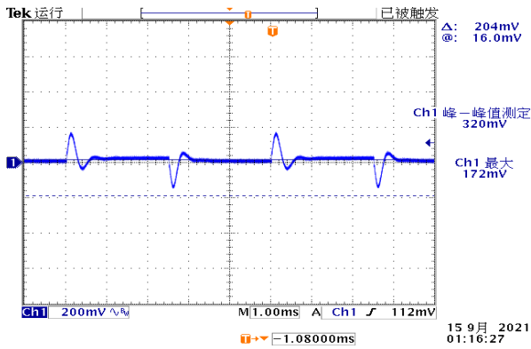
Figure 4, 25% - 50% load dynamic
