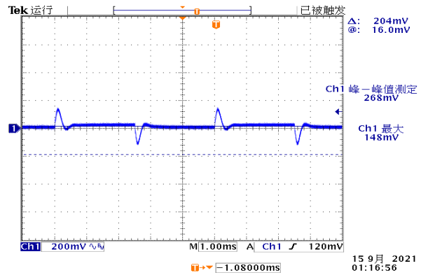
Figure 5, 50% - 75% load dynamic
