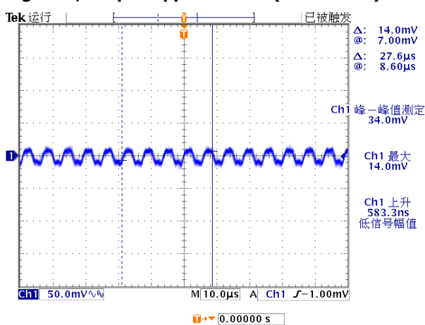
Figure 7, Output ripple & noise (Iout = 10A)
