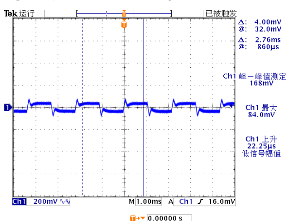
Figure 5, 50% - 75% load dynamic
