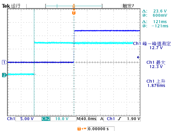
Figure 6, Output voltage established (Iout = 8A)
