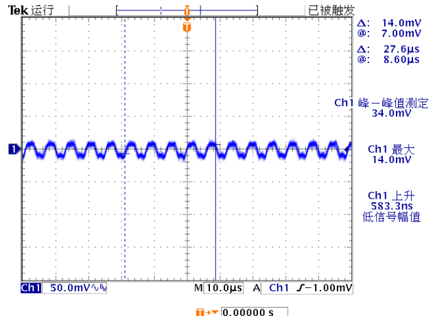
Figure 7, Output ripple & noise (Iout = 8A)
