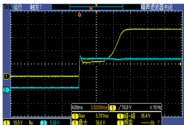
Figure 6, Output voltage established (Iout = 6A)
