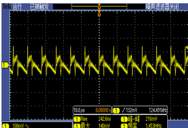
Figure 7, Output ripple & noise (Iout = 6A)
