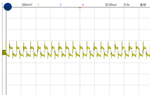
Figure 7, Output ripple & noise ( I_{out} = 10\text{A} )
