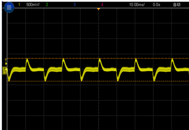
Figure 4, 25% - 50% load dynamic
