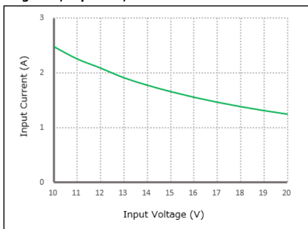
Figure 3, Input V-I, Iout=1A
