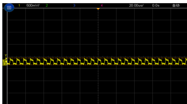
Figure 7, Output ripple & noise ( I_{out} = 1\text{A} )
