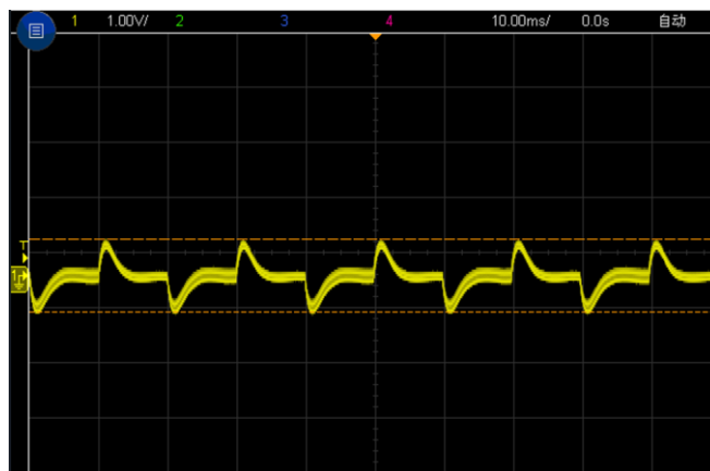
Figure 5, 50% - 75% load dynamic
