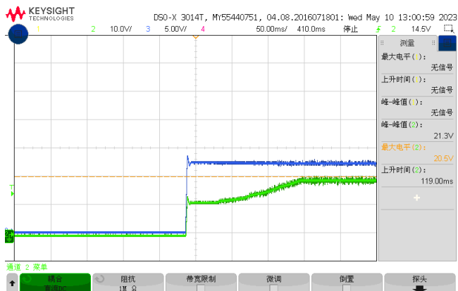
Figure 6, Output voltage established ( I_{out} = 30\text{A} )
