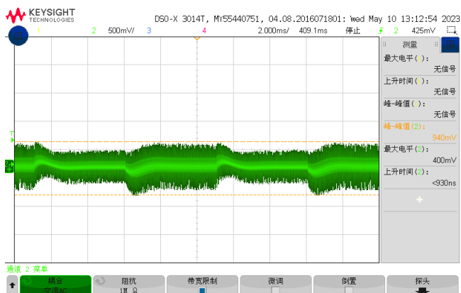
Figure 4, 25% - 50% load dynamic
