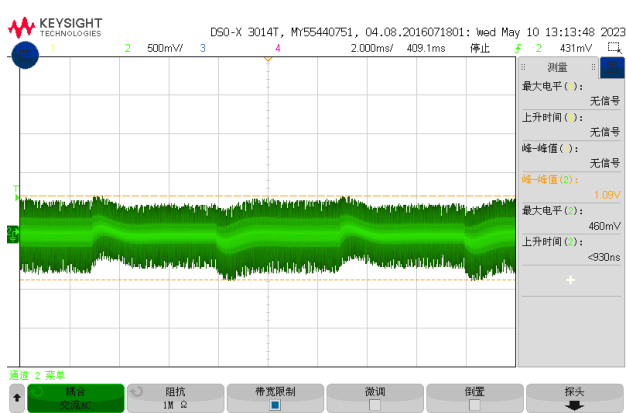
Figure 5, 50% - 75% load dynamic
