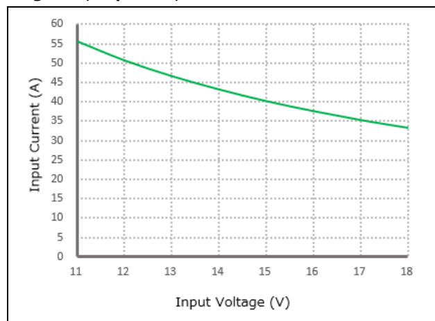
Figure 3, Input V-I, I_{out}=30\text{A}
